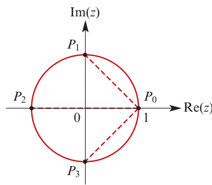
Fourth roots of unity
