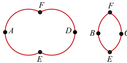
A cycle splitting for G
