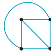
K_4 without edges crossing
